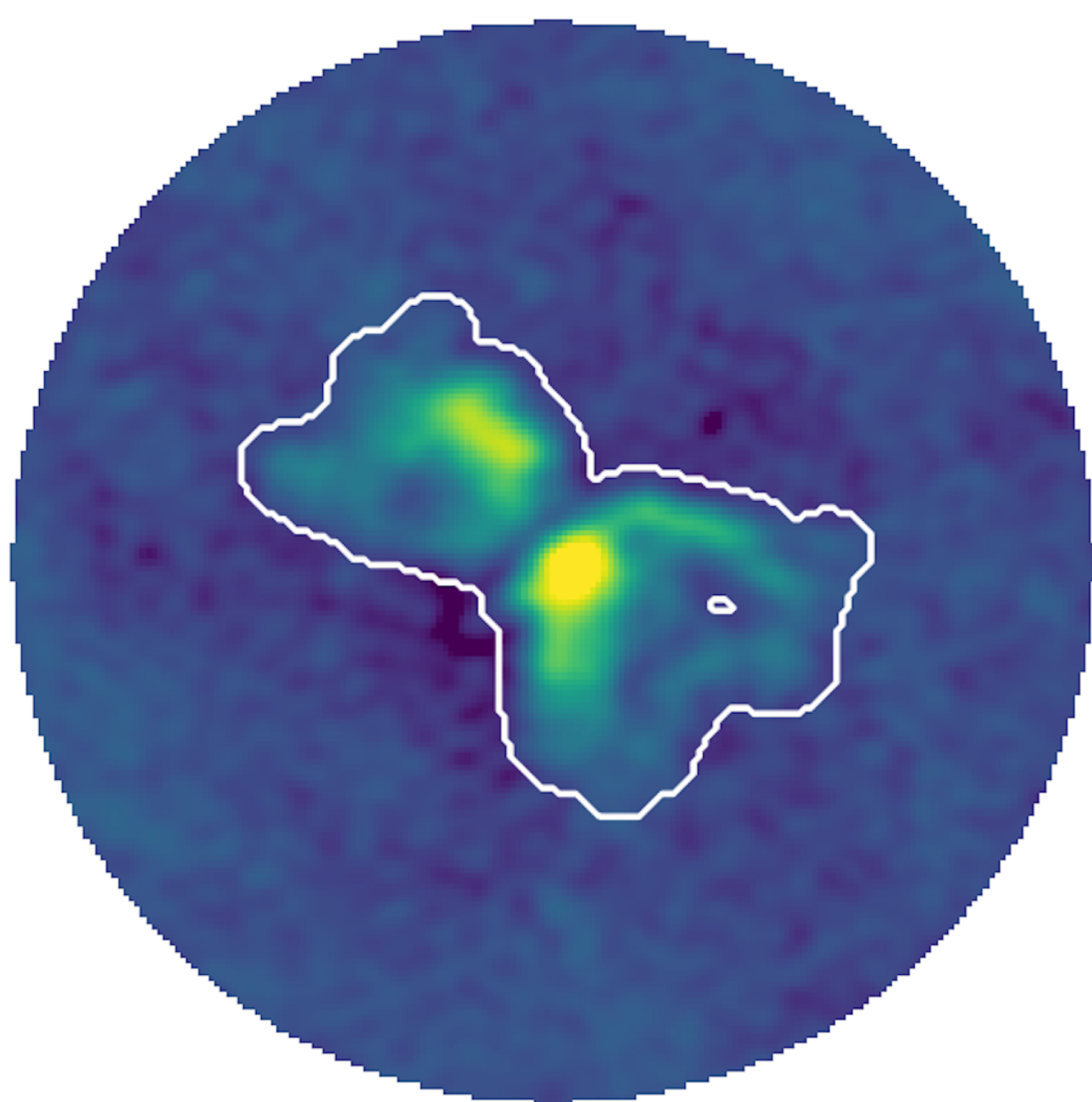
Figure: Channel map of an ALMA 12m data set. The contour shows the mask produced with automated masking. Credit: A. Kepley (NRAO).
